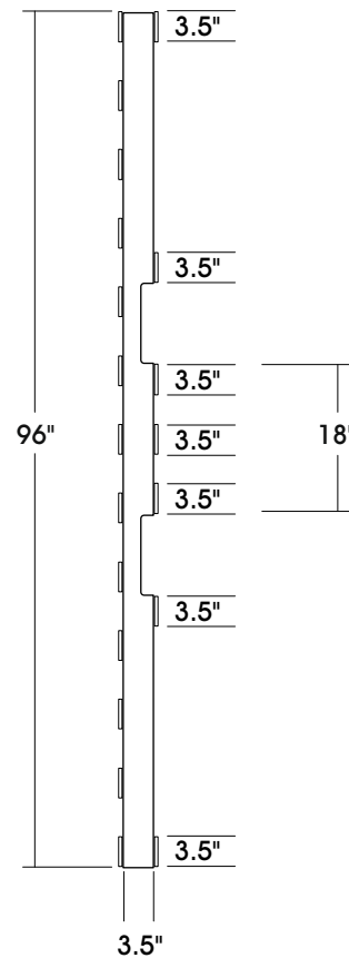
SIDE VIEW
